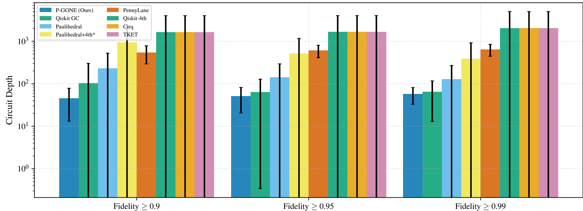
Circuit Depth at Fidelity Thresholds
