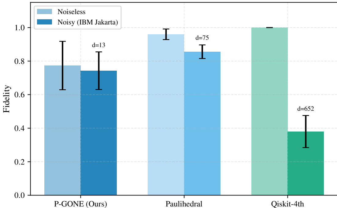
Noisy Hardware: Fidelity Comparison
