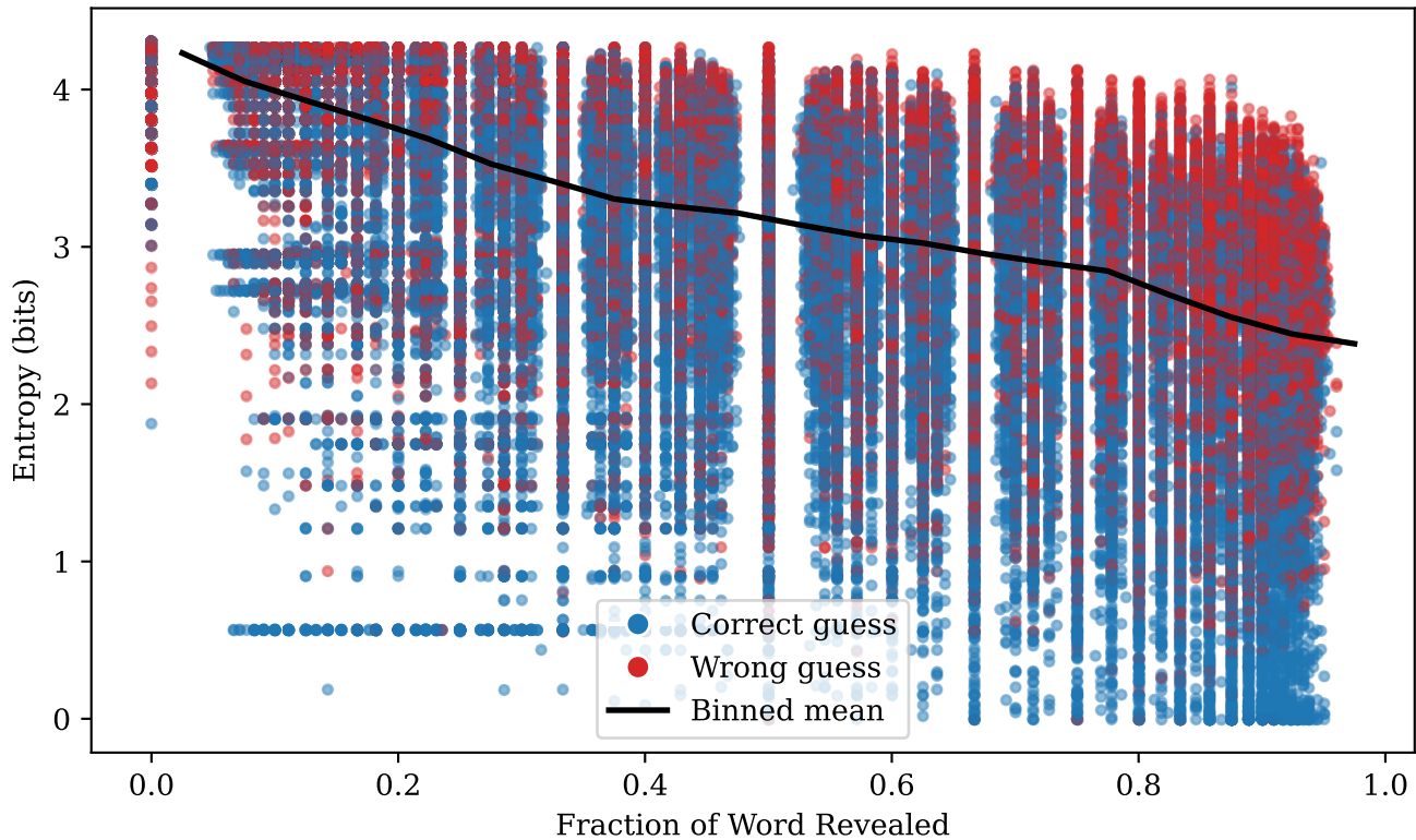
Solver Entropy vs. Game Progress
