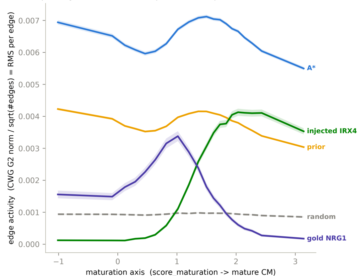
CWG per-edge (L2-consistent, /sqrt n) — A* vs prior, count confound removed
