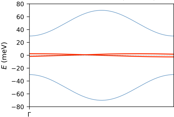
Moire band structure ( \theta = 1.1^\circ )
