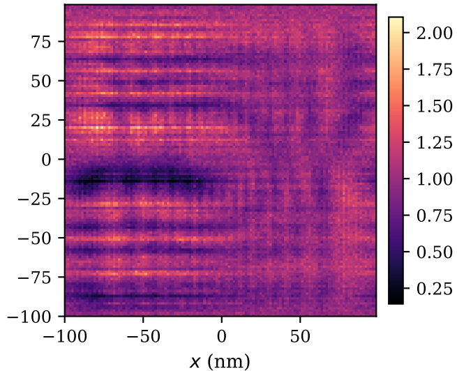
|\psi|^2 at t = 1 ps
