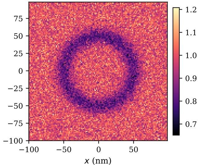
|\psi|^2 at t = 0
