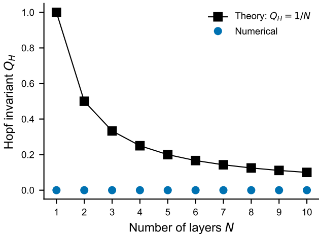
Hopf invariant: 1/N quantization
