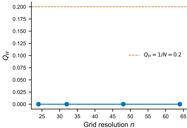
(a) Convergence of Hopf invariant
