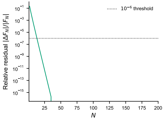
(b) Convergence rate
