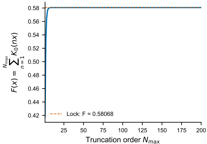
(a) Partial sum convergence
