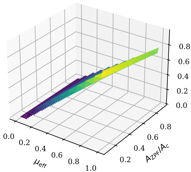
(a) Hall staircase vs vacuum coupling
