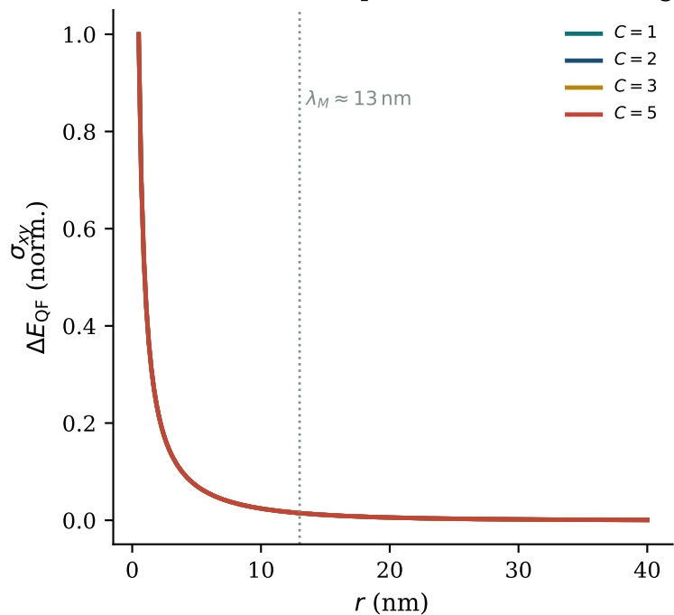
(b) Quantum atmosphere (moiré screening)
