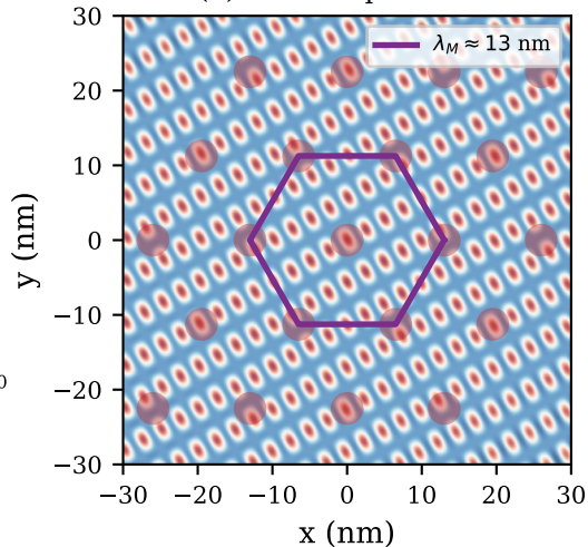
(b) Moiré superlattice
