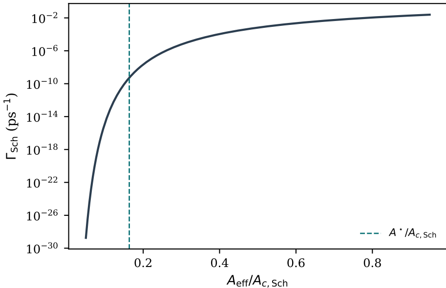
Schwinger rate (new E_{\text{vac}} , democratic |\lambda_{\text{min}}| )
