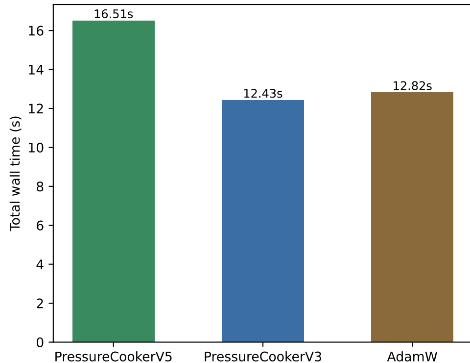
Training time — 60 steps (10 warmup excluded from per-step time)
