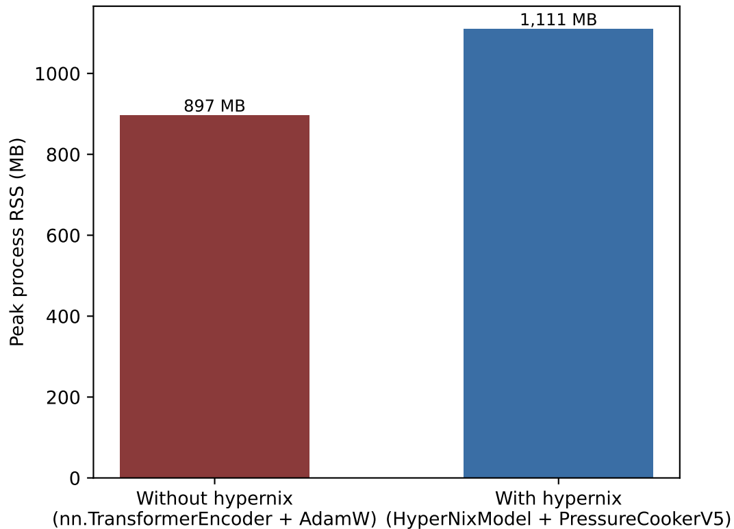
RAM usage — 60 steps, 4L/256H model
