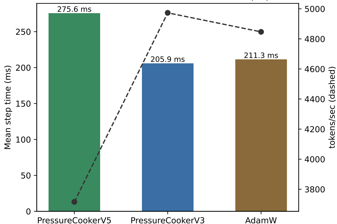
PressureCookerV5 vs V3 vs AdamW — step speed
