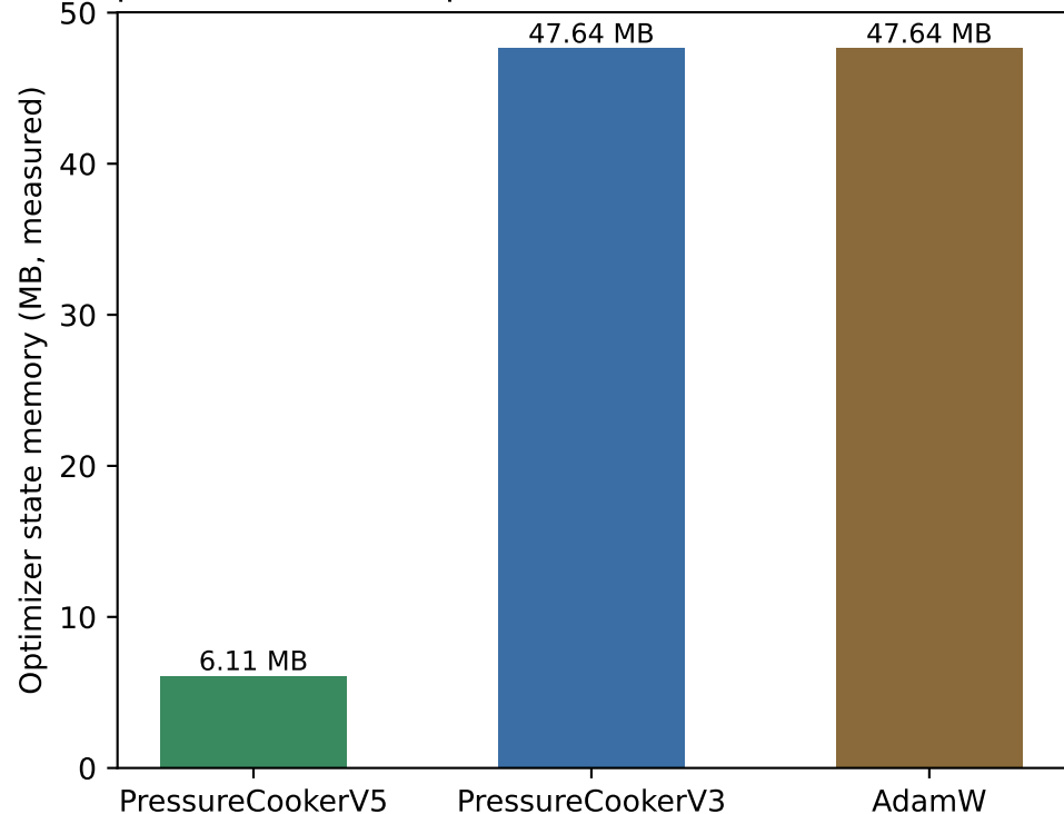
Optimizer state footprint (momentum/curvature buffers)
