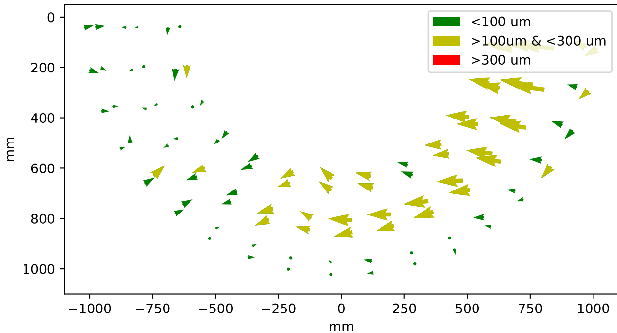
DD12-O-103, 2S Positions, Bottom side
