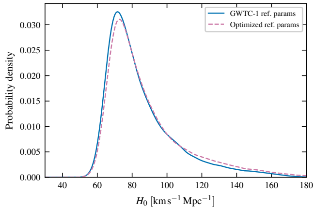
(b) Heterodyne reference sensitivity
