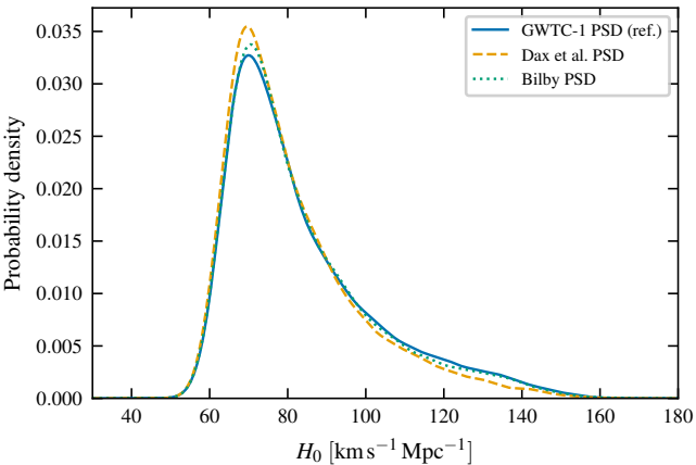
(a) PSD sensitivity (TaylorF2)
