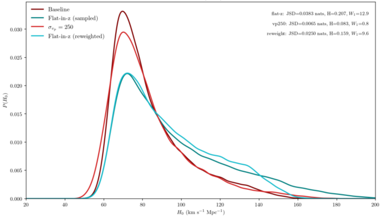
Prior Sensitivity: TaylorF2
