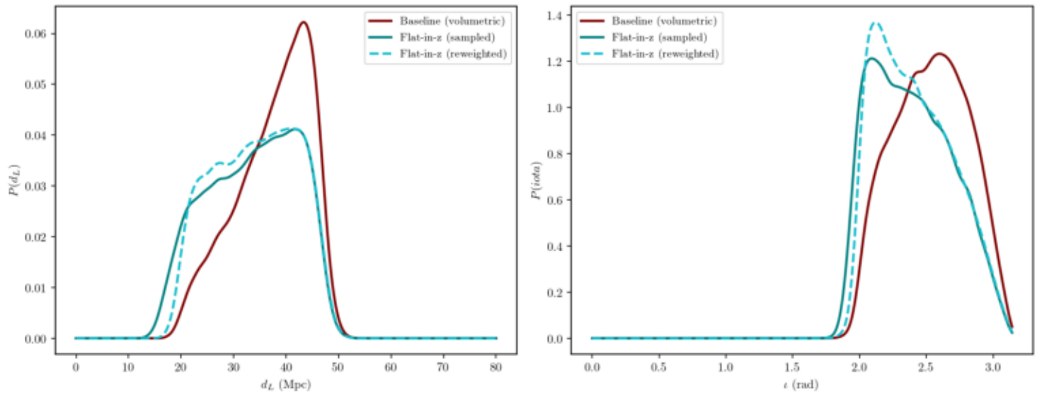
Reweighted vs Directly Sampled: TaylorF2
