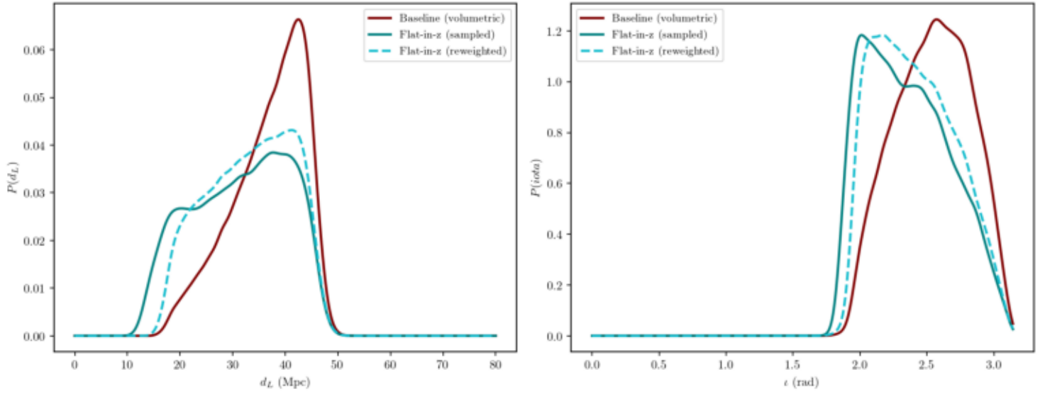
Reweighted vs Directly Sampled: IMRPhenomD_NRTidalv2
