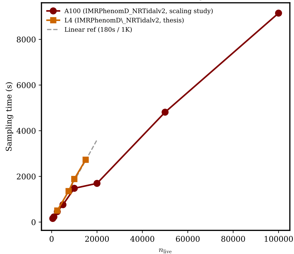
Runtime scaling
