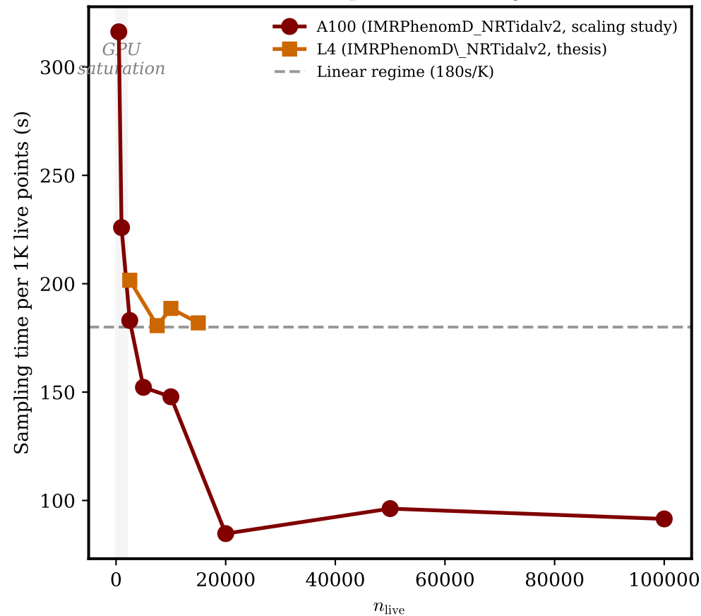
Per-live-point efficiency
