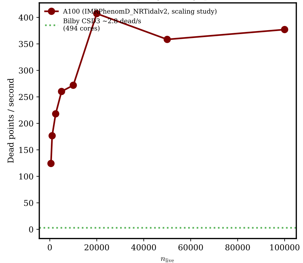
Sampling throughput
