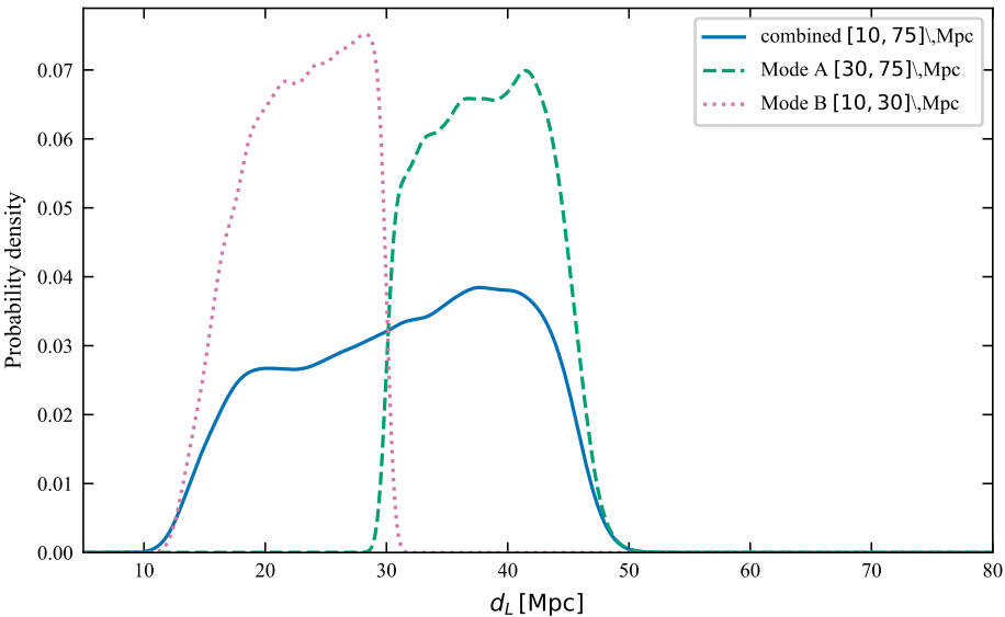
GW170817 d_L marginals by mode
