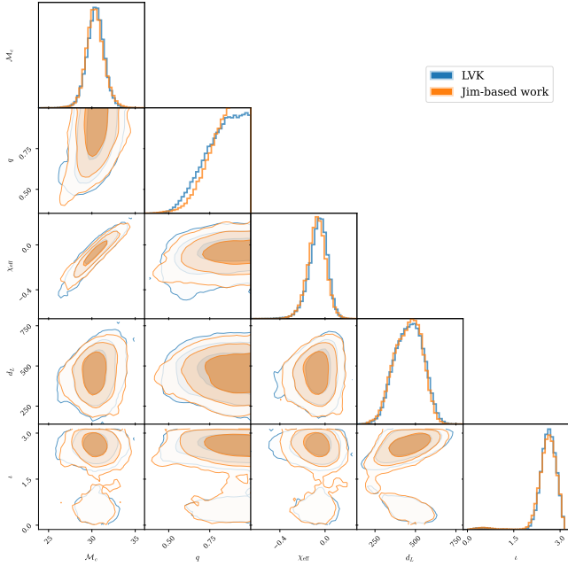
Figure 1. GW150914 validation: corner overlay of the LVK GWTC-2.1 IMRPhenomXPHM posterior and our heterodyned IMRPhenomXPHM run at n_{\text{live}} = 5000 . Both legend entries use the same waveform, so the panels show a like-for-like reproduction.
