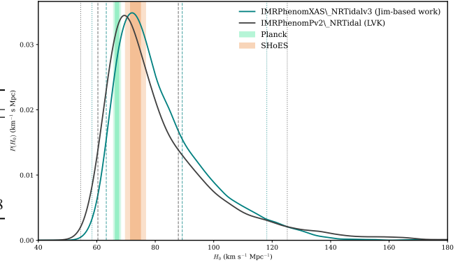
Figure 2. GW170817 H_0 posterior under the LVK-bounds baseline prior for the two NR-calibrated tidal waveforms used as primary/anchor (IMRPhenomXAS_NRTidalv3, IMRPhenomD_NRTidalv2), plus the GWTC-1 IMRPhenomPv2_NRTidal posterior mapped through this work’s standard-siren likelihood of equation 2. Vertical markers are sample-derived 68 per cent HPD bounds. The Planck \Lambda CDM and SHoES distance-ladder values are shown for context. The TaylorF2 and IMRPhenomPv2 (no tides) family checks are reported in Table 2 and retained in the public test suite, but are not promoted to this figure.
