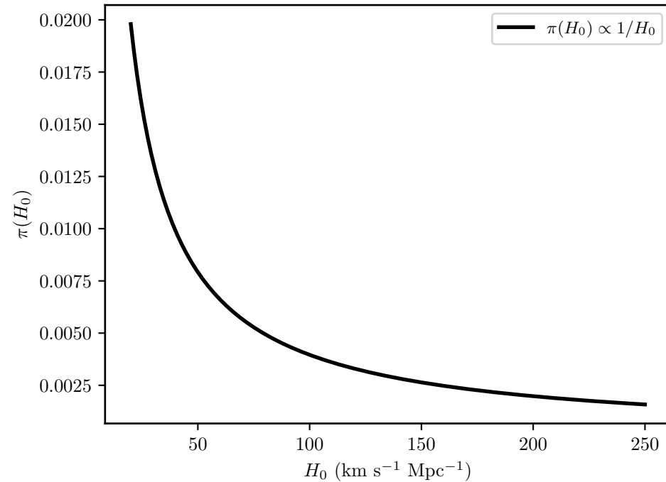
H_0 Prior (log-uniform)
