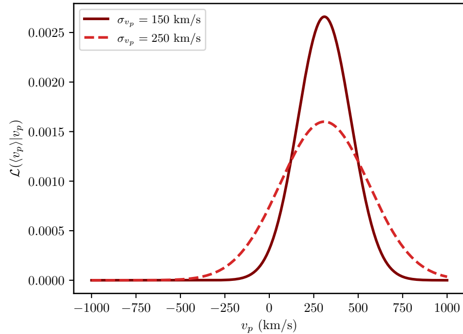
Peculiar Velocity Likelihood
