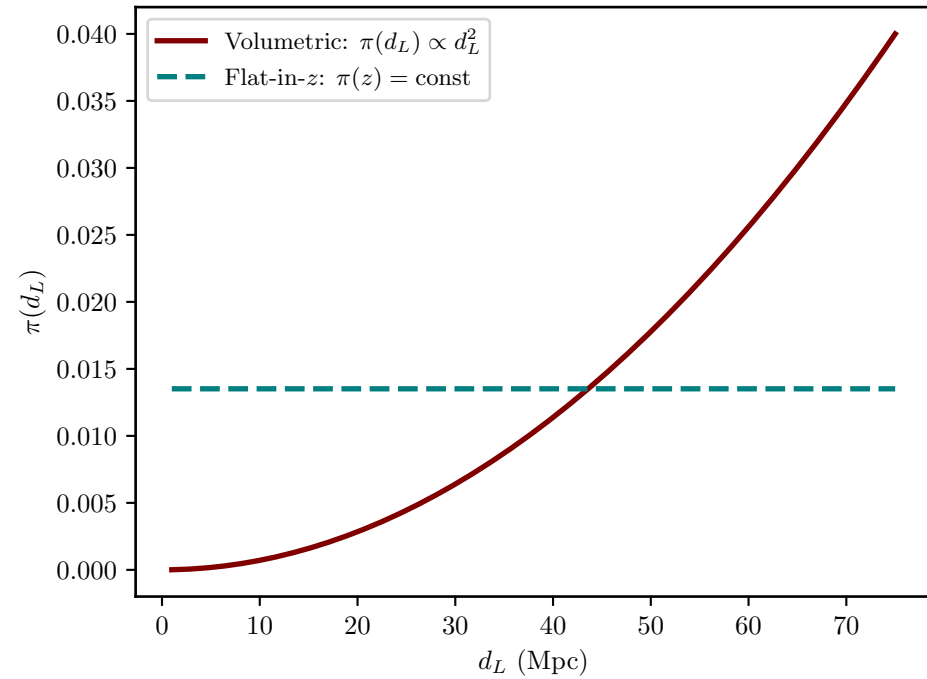
Distance Prior
