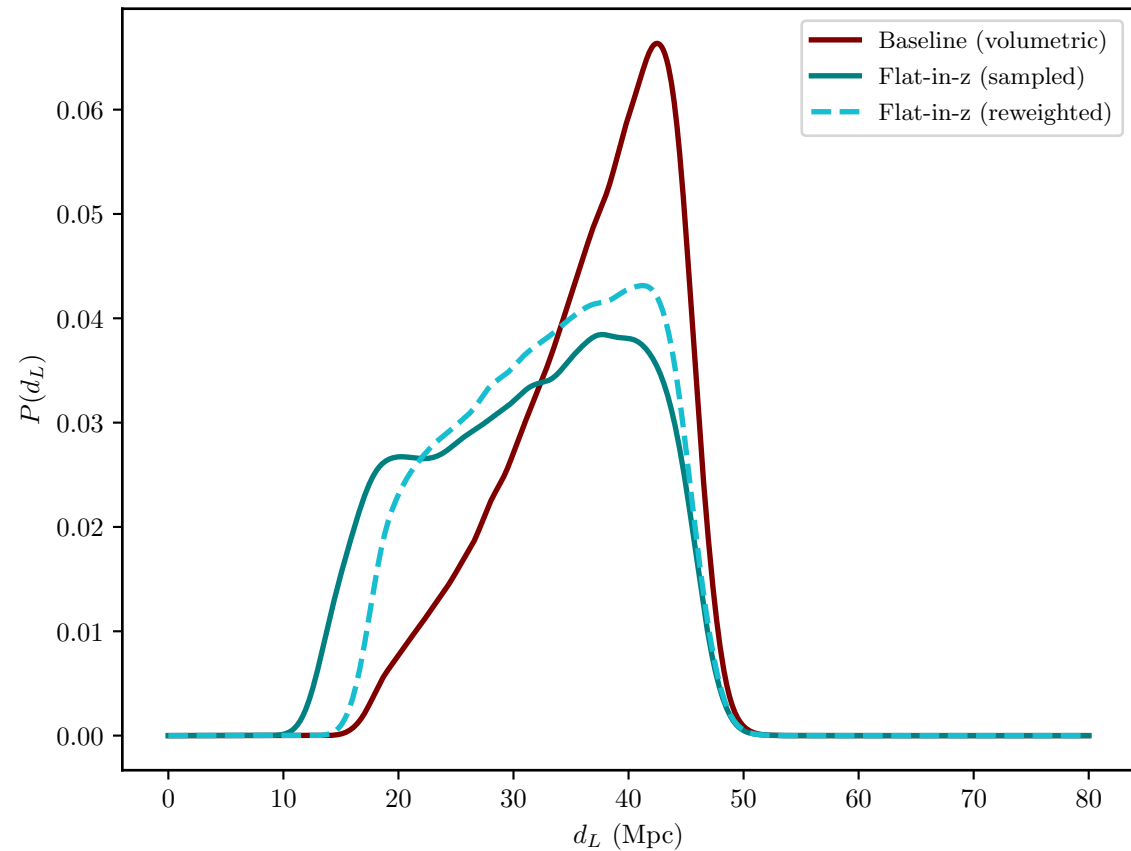
Reweightd vs Directly Sampled: IMRPhenomD_NRTidalv2
