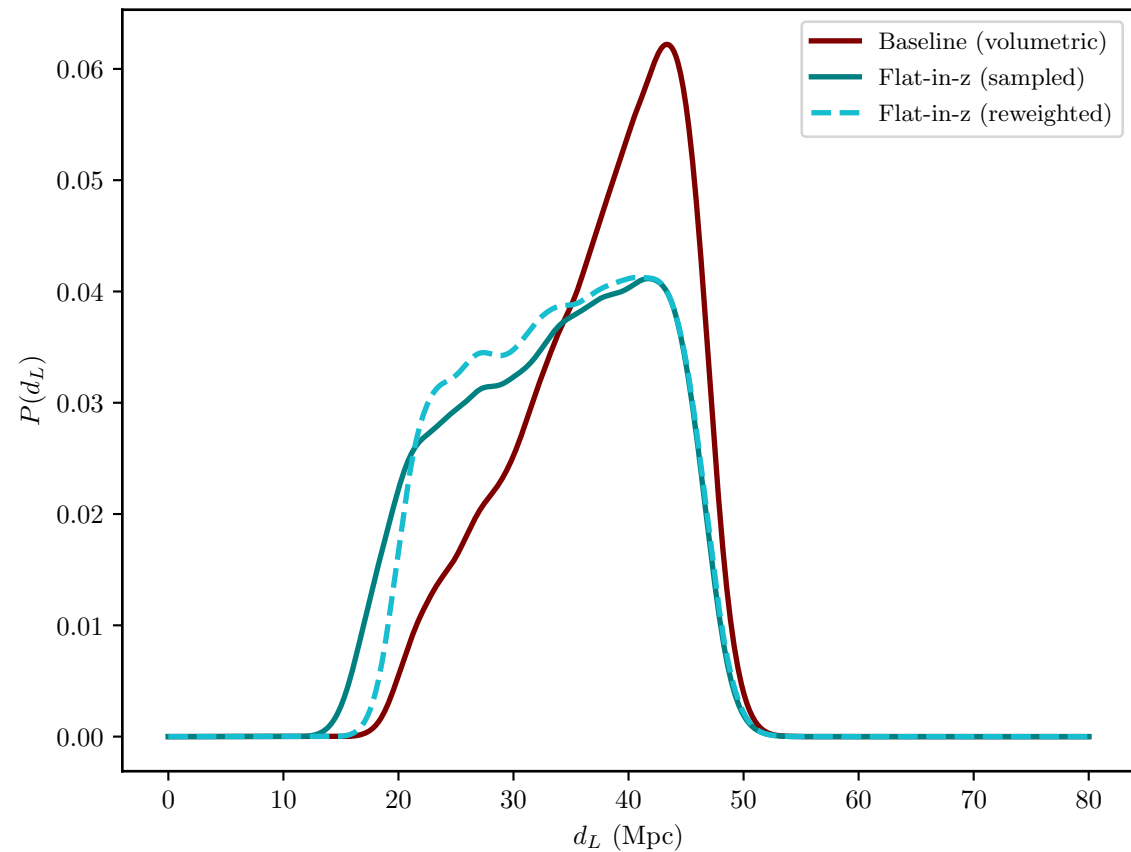
Reweightd vs Directly Sampled: TaylorF2
