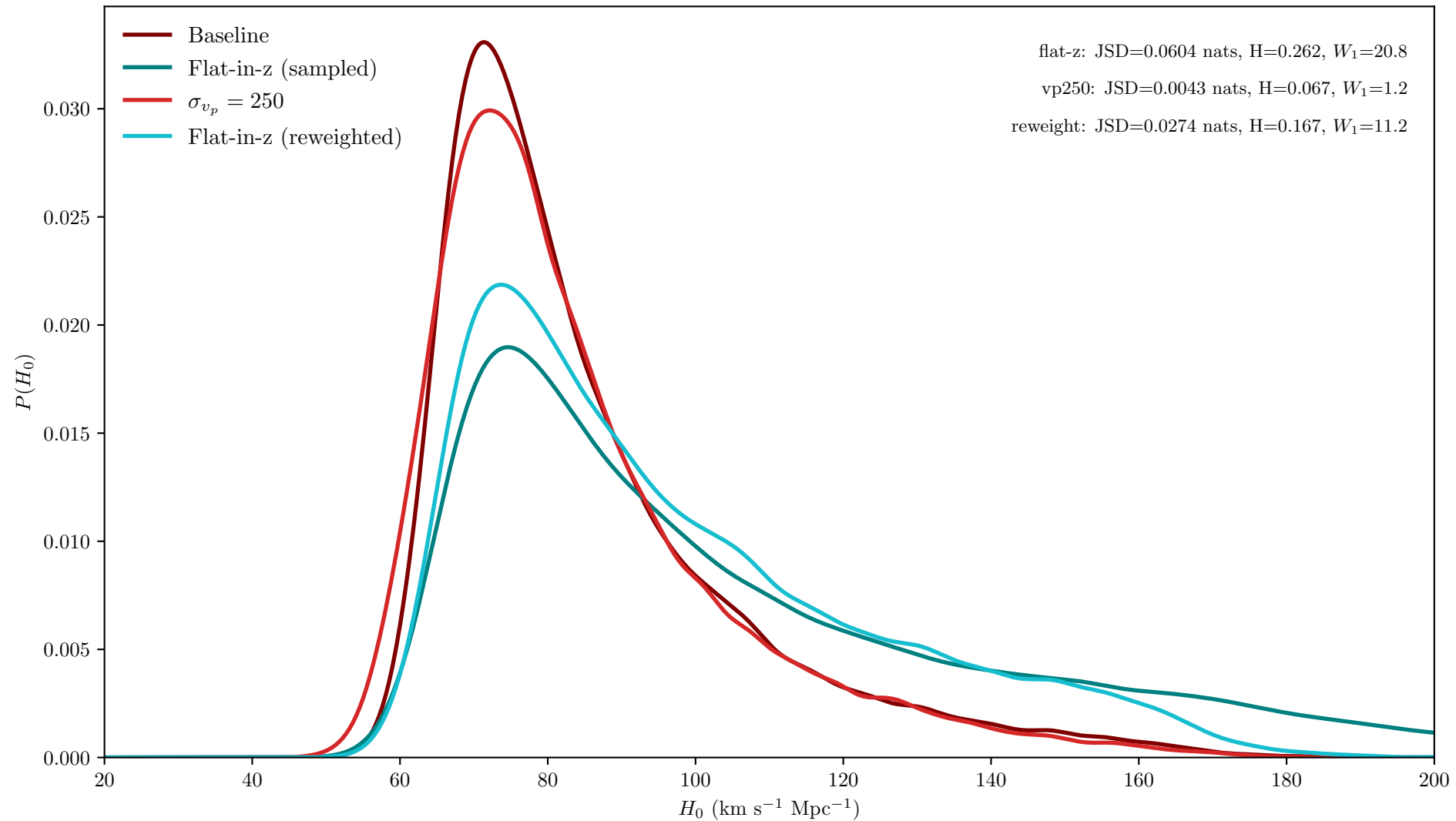
Prior Sensitivity: IMRPhenomD_NRTidalv2
