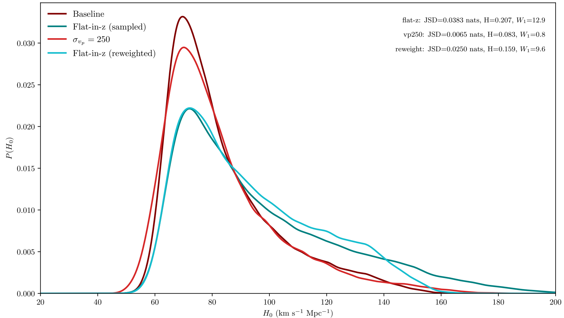
Prior Sensitivity: TaylorF2
