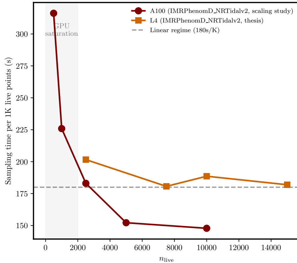
Per-live-point efficiency
