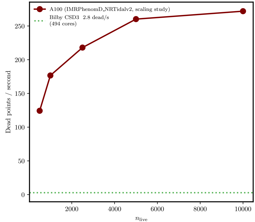
Sampling throughput
