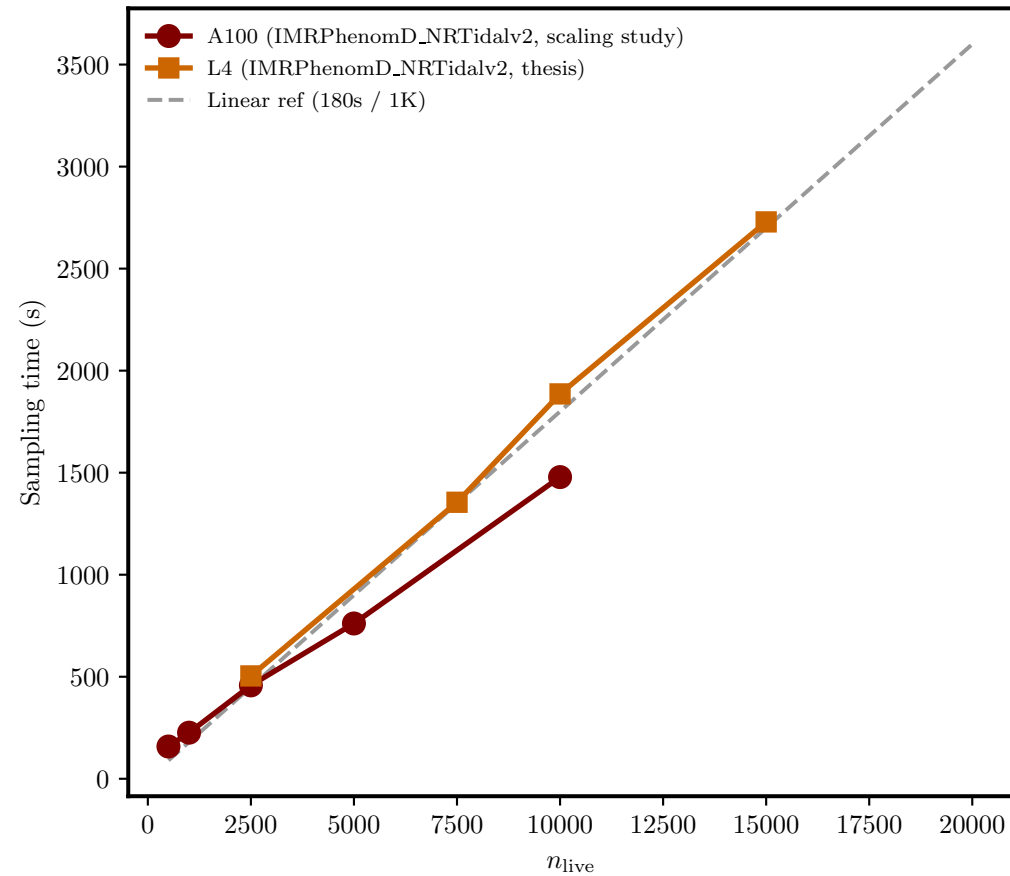
Runtime scaling
