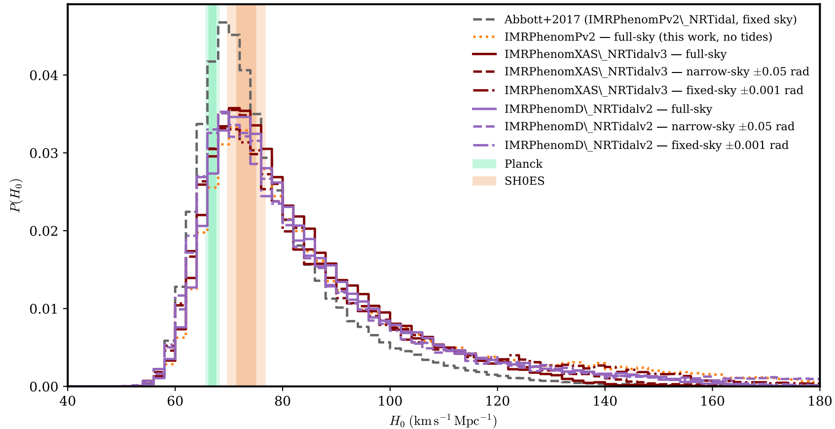
Abbott+2017 reproduction study: sky-restriction and waveform effects on H_0
