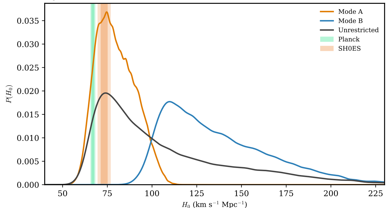
Figure 3b KDE bw= \times 0.4
