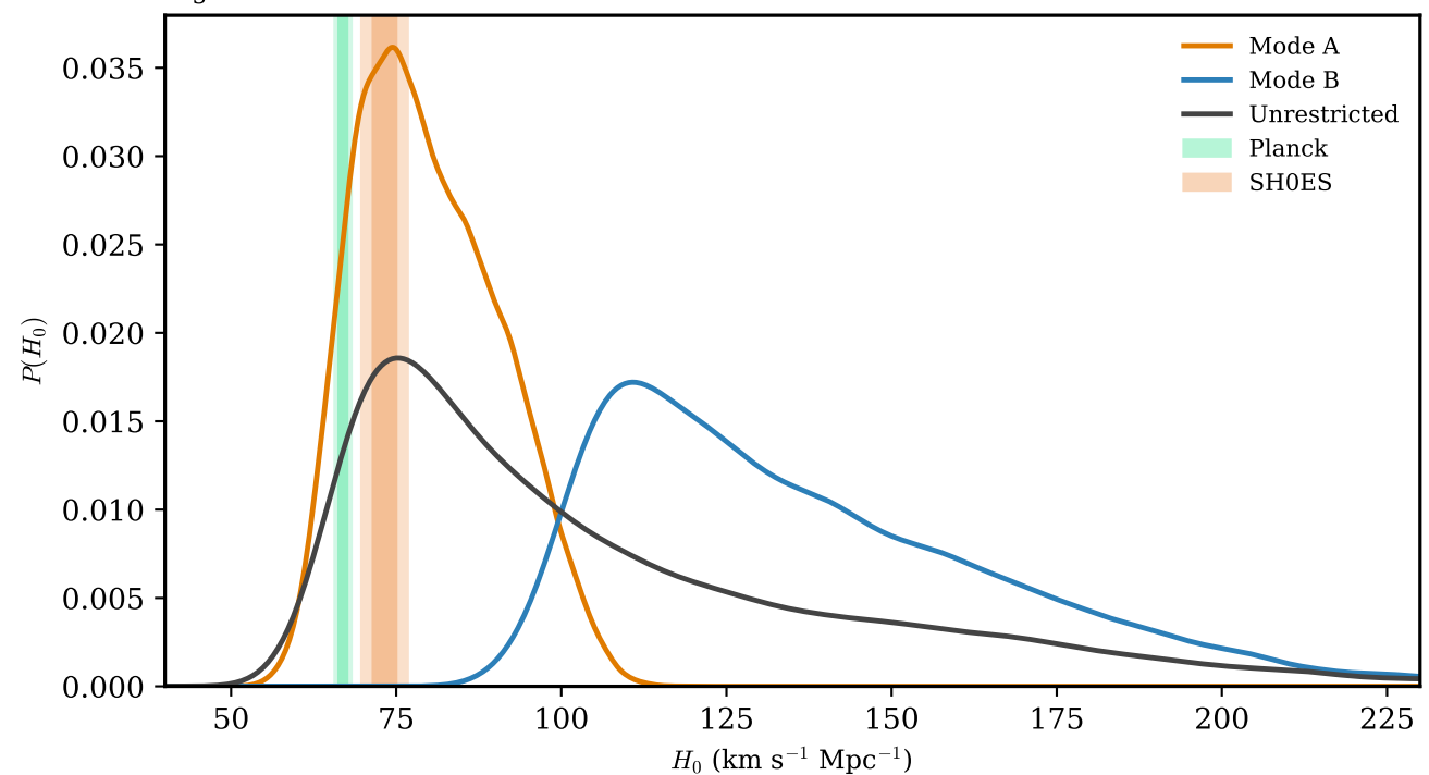
Figure 3b KDE bw= \times 0.6
