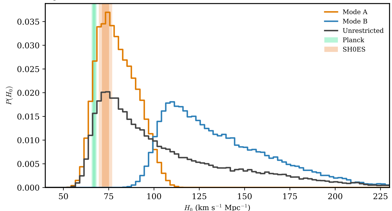
Figure 3b KDE bw=Silverman
