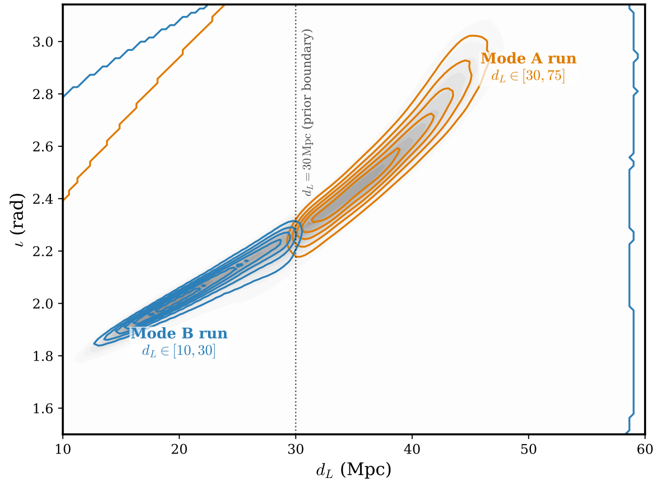
(a) Joint ( d_L, \iota ) posterior, flat-in- z
