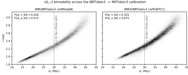
Figure 4. Cross-waveform check on the (d_L, \iota) bimodality: weighted joint posteriors from the unrestricted direct uniform-in- d_L runs at IMRPhenomD_NRTidalv2 (left; Mode-B-anchored heterodyne reference) and IMRPhenomXAS_NRTidalv3 (right; default GWTC-1 reference). Both show the same two-peak structure with the Mode-B region d_L < 30 Mpc carrying 0.428 (IMRPhenomD_NRTidalv2) and 0.325 (IMRPhenomXAS_NRTidalv3) of the posterior weight: the bimodality is robust across the NRTidalv2 \rightarrow NRTidalv3 calibration. The smaller IMRX Mode-B weight is consistent with the tighter upper H_0 tail under NRTidalv3 reported in Section 4.1.
