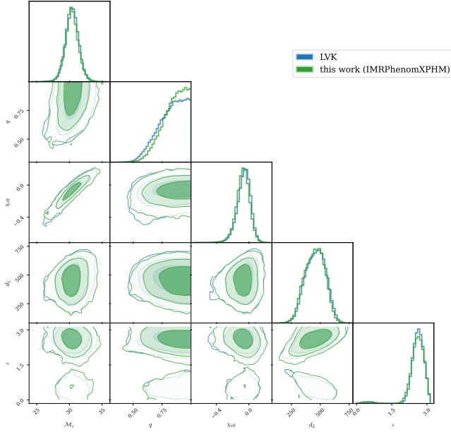
Figure 1. GW150914 validation: corner overlay of the LVK GWTC-2.1 IMR-PhenomXPHM posterior (Abbott et al. 2024; LIGO Scientific Collaboration et al. 2022) and our heterodyned IMRPhenomXPHM run at n_{\text{live}} = 8000 , n_{\text{mcmc}} = 160 . The two posteriors overlap throughout the recovered support; our component-mass prior [5, 100] M_{\odot} encompasses the LVK [10, 80] M_{\odot} range without adding posterior mass at the boundaries.
