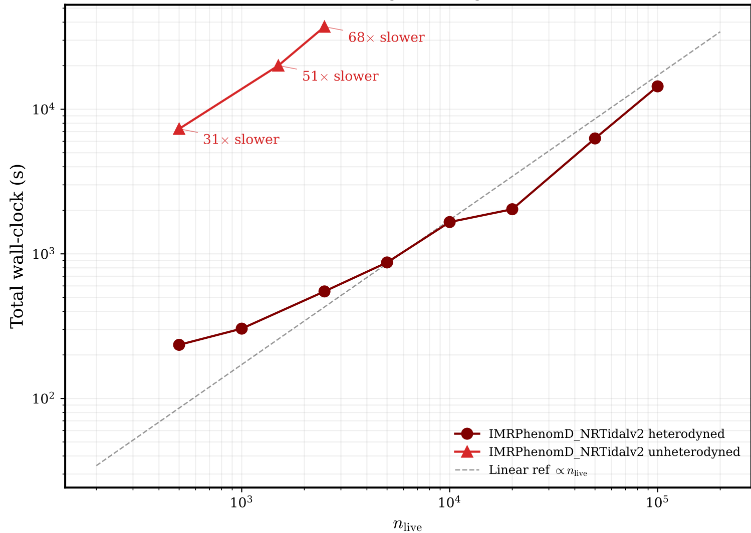
Runtime scaling, all configurations
