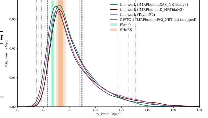
Figure 2. GW170817 H_0 posterior for the three-waveform set of Table 2: IMRPhenomXAS_NRTidalv3 (primary, LVK-bounds baseline), IMRPhenomD_NRTidalv2 (anchor, LVK-bounds baseline), and TaylorF2 (family check, default-mass baseline), plus the GWTC-1 IMRPhenomPv2_NRTidal posterior mapped through this work’s standard-siren likelihood of equation 2. Vertical markers are 68 per cent and 95 per cent HPD bounds derived from a weighted KDE; sample-derived HPDs are reported in Table 2. The Planck \Lambda CDM and SHoES distance-ladder values are shown for context. The IMRPhenomPv2 (no tides) cross-check is reported inline in Section 4.1 and retained in the public test suite.
