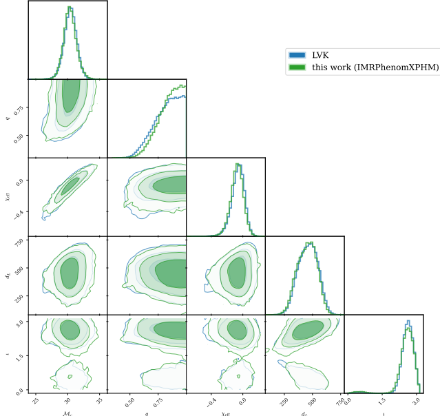
Figure 1. GW150914 validation: corner overlay of the LVK GWTC-2.1 IMRPhenomXPHM posterior and our heterodyned IMRPhenomXPHM run at n_{\text{live}} = 8000 , n_{\text{mcmc}} = 160 . Both legend entries use the same waveform, so the panels show a like-for-like reproduction.
