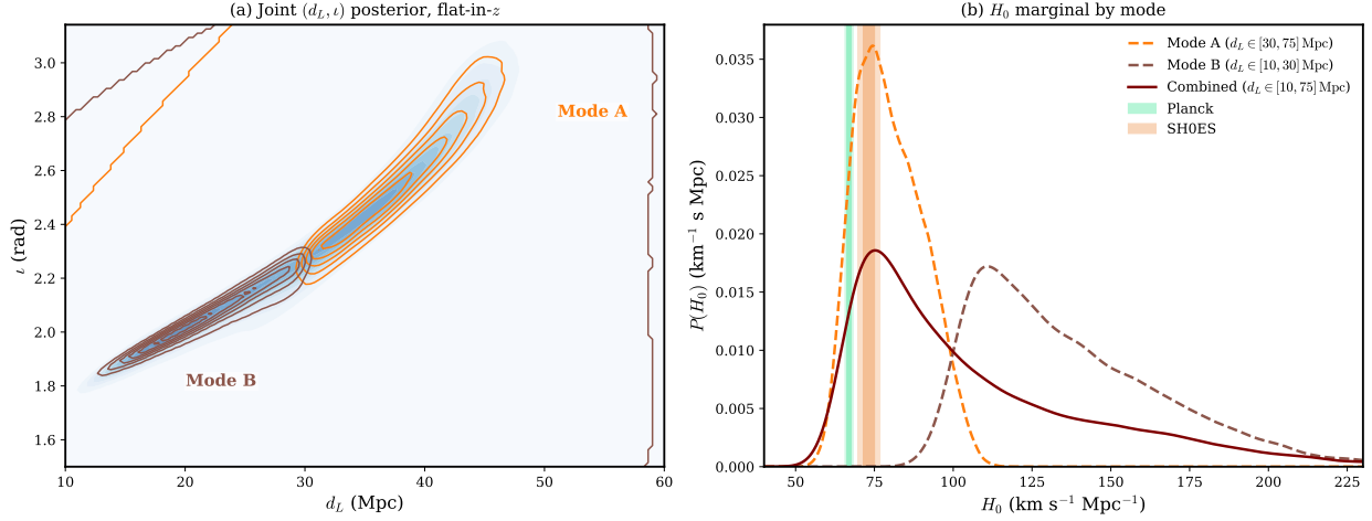
Figure 5. The d_L – \iota bimodality in the GW170817 flat-in-redshift posterior. Left: joint (d_L, \iota) posterior from the unrestricted d_L \in [10, 75] Mpc run (Mode-B-anchored heterodyne reference), with the prior-restricted Mode-A and Mode-B contours overlaid. Right: per-mode H_0 marginals as weighted step-histograms. The Planck \Lambda CDM and SH0ES distance-ladder bands are shown for context; this work is itself a GW170817 reanalysis, so the LVK GW170817 band is uninformative here and is not included.
