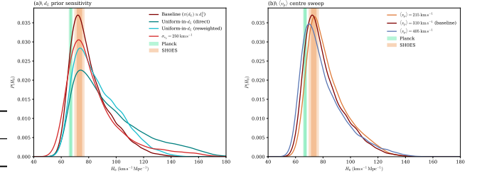
Figure 2. Prior-sensitivity comparison for IMRPhenomXAS_NRTidalv3. Left panel (a): weighted step-histograms of H_0 under the four distance-prior variants of Section 2.4 (volumetric baseline, direct uniform-in- d_L , reweighted uniform-in- d_L , and \sigma_{v_p} = 250 \text{ km s}^{-1} ). The directly sampled uniform-in- d_L posterior places substantially more mass at high H_0 than the reweighted estimate, despite both targeting the same prior. Right panel (b): peculiar-velocity centre sweep — H_0 posteriors for \langle v_p \rangle \in \{215, 310, 405\} \text{ km s}^{-1} at fixed \sigma_{v_p} = 150 \text{ km s}^{-1} (s18 runs). The published Abbott+2017 H_0 = 70^{+12}_{-8} \text{ km s}^{-1} \text{ Mpc}^{-1} band (Abbott et al. 2017b) is shown in panel (a) as a vertical reference. Planck \Lambda\text{CDM} and SH0ES distance-ladder bands are shown in both panels.
