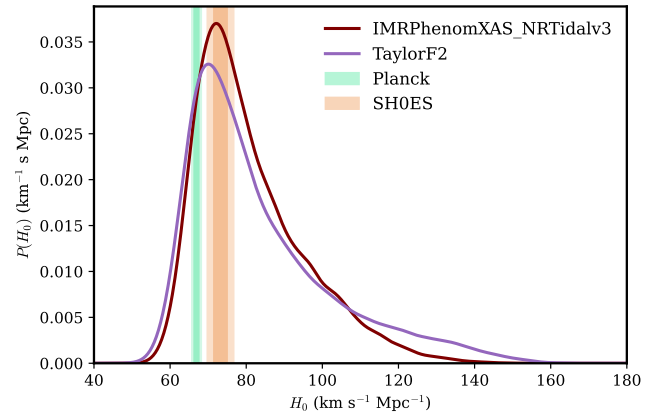
Figure 5. GW170817 H_0 posterior for IMRPhenomXAS_NRTidalv3 (primary) and TaylorF2 (family check) on the LVK-matched prior, shown as Silverman-bandwidth kernel-density estimates; the sample-derived 68 and 95 per cent HPDs (computed from the weighted samples, no KDE) are reported in Table 4. The Planck \Lambda CDM and SH0ES distance-ladder values are shown for context.
