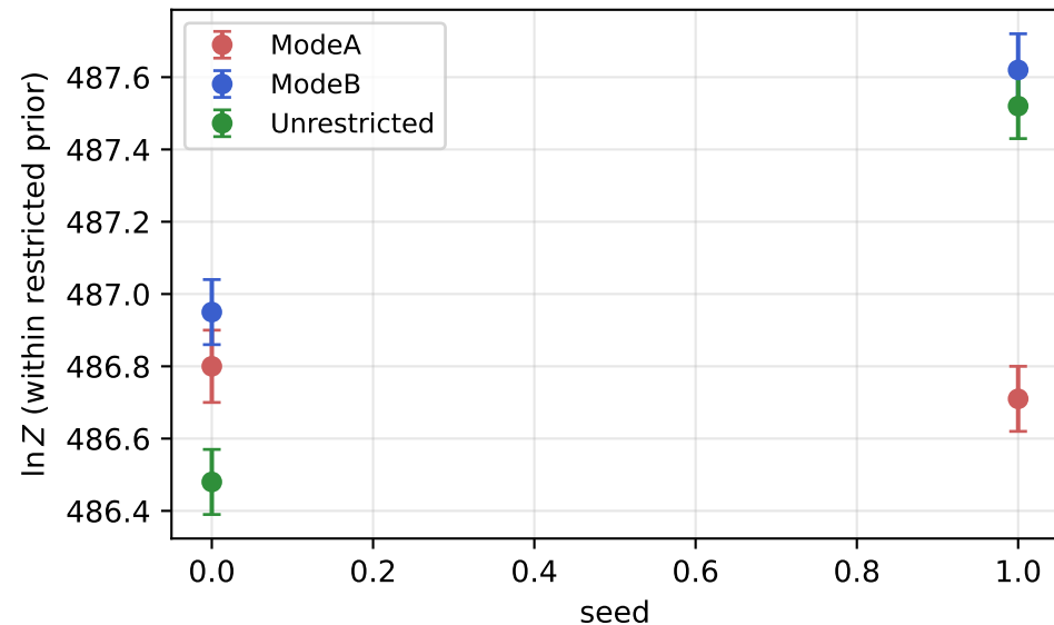
(a) Per-seed \ln Z for the three bimodality runs
