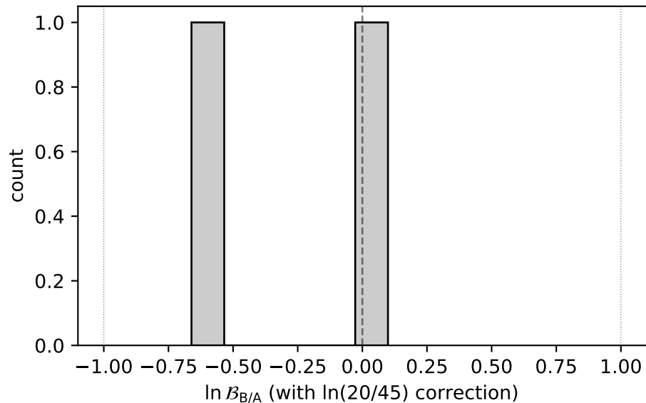
(b) Per-seed Mode-B/Mode-A Bayes factor distribution
