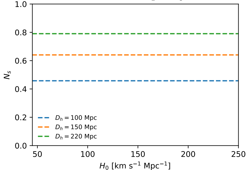
(a) as run: uniform in d_L \Rightarrow N_s constant
