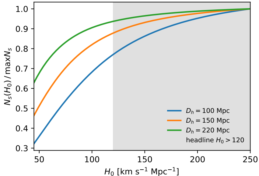
(b) genuine flat-in-z: N_s(H_0) (normalised)
