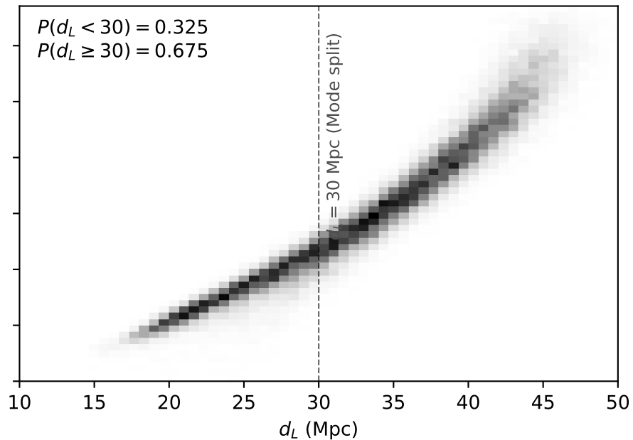
IMRX/NRTidalv3 (refGWTC1)
