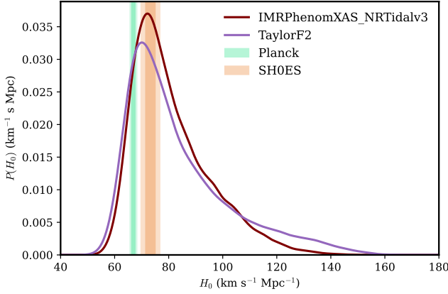
Figure 5. GW170817 H_0 posterior for IMRPhenomXAS_NRTidalv3 and TaylorF2 on the LVK-matched prior, shown as Silverman-bandwidth kernel-density estimates; the sample-derived 68 and 95 per cent HPDs (computed from the weighted samples, no KDE) are reported in Table 4. The Planck \Lambda CDM and SH0ES distance-ladder values are shown for context.
