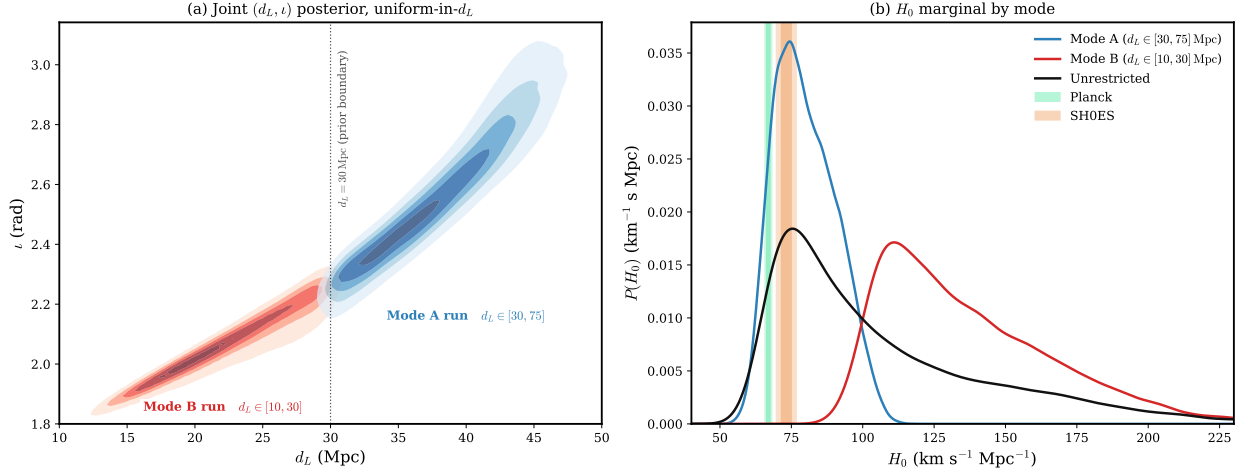
Figure 4. The d_L – \iota bimodality in the GW170817 uniform-in- d_L posterior. Left: joint (d_L, \iota) posterior from the unrestricted d_L \in [10, 75] Mpc run (Mode-B-anchored heterodyne reference); the prior-restricted Mode-A and Mode-B contours from the two separate restricted-prior runs are overlaid in distinct colours, with the d_L = 30 Mpc prior boundary marked. Right: per-mode H_0 marginals as Silverman-bandwidth kernel-density estimates. The Planck \Lambda CDM and SH0ES distance-ladder bands are shown for context.
