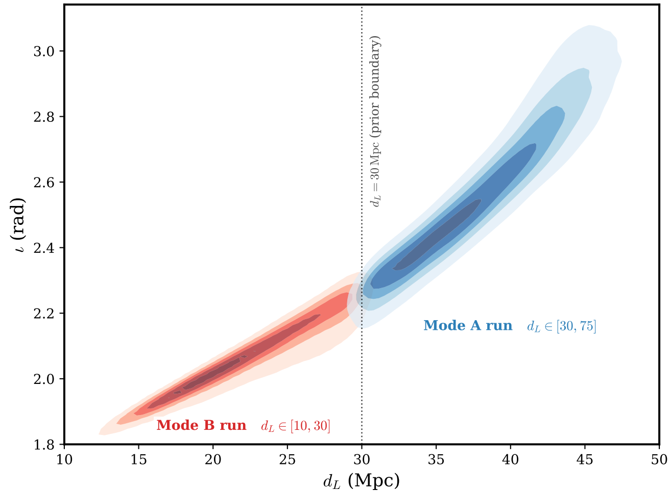
(a) Joint ( d_L, \iota ) posterior, uniform-in- d_L
