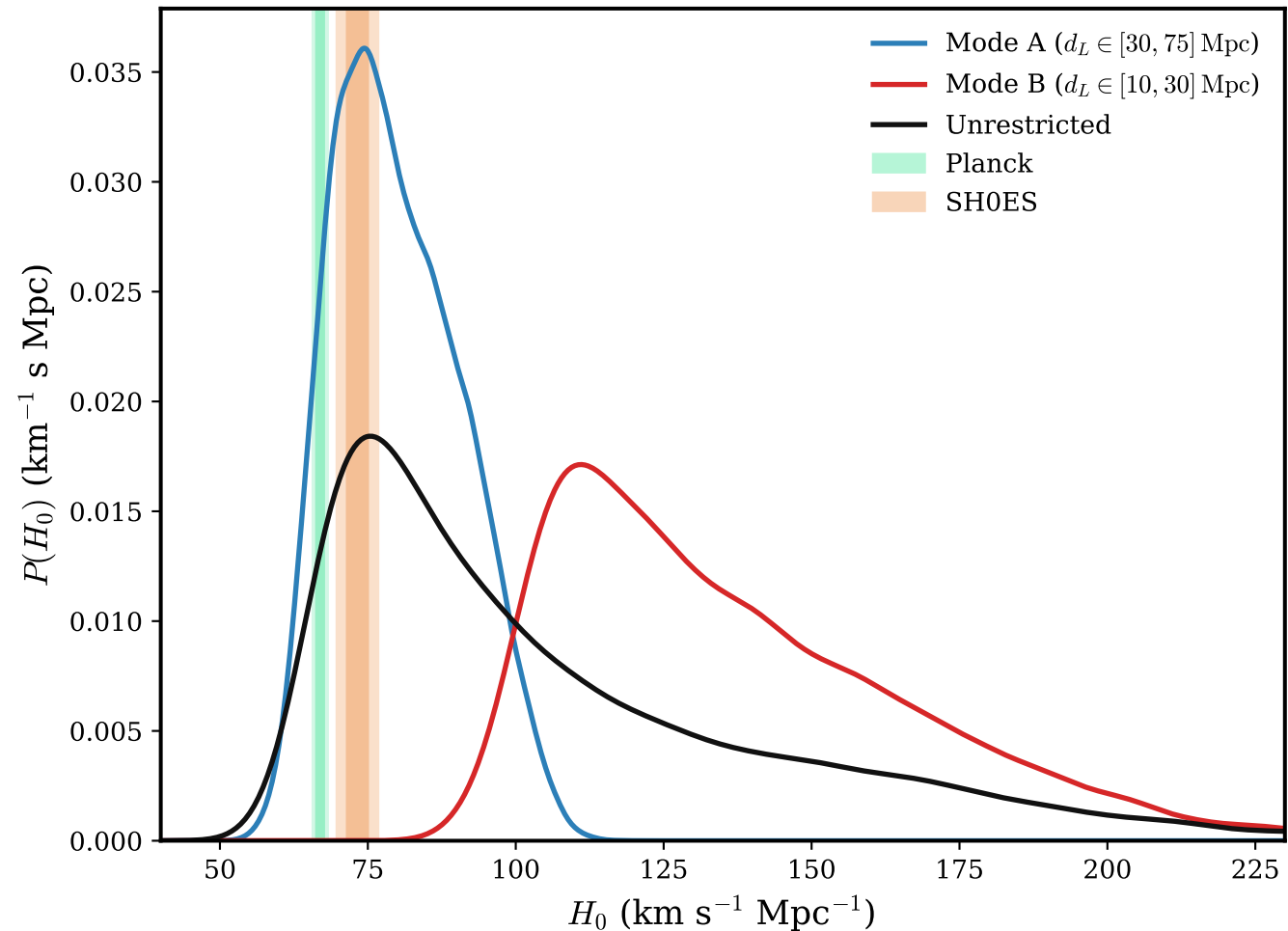
(b) H_0 marginal by mode
