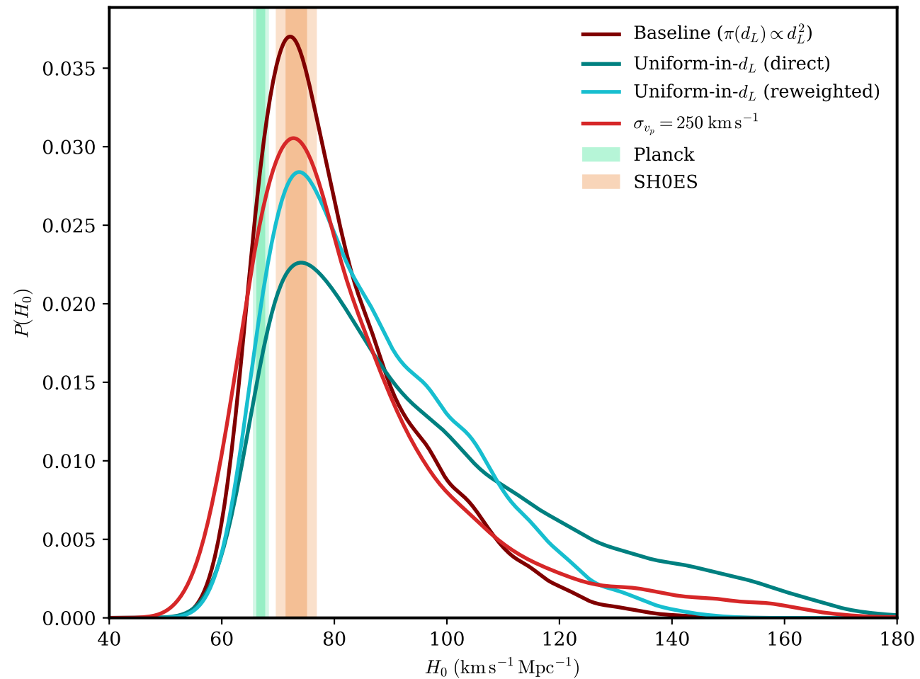
(a) d_L prior sensitivity
