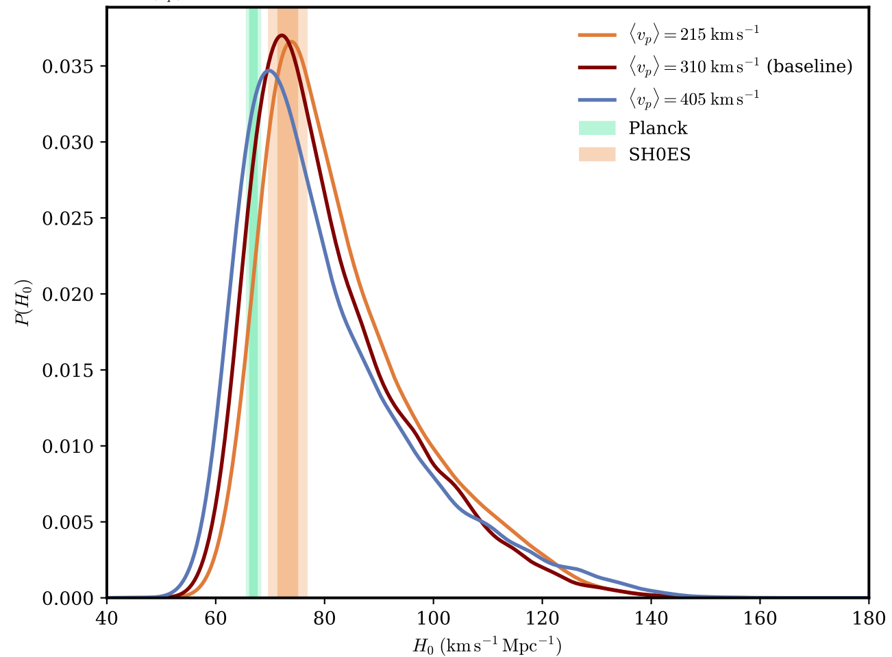
(b) \langle v_p \rangle centre sweep
