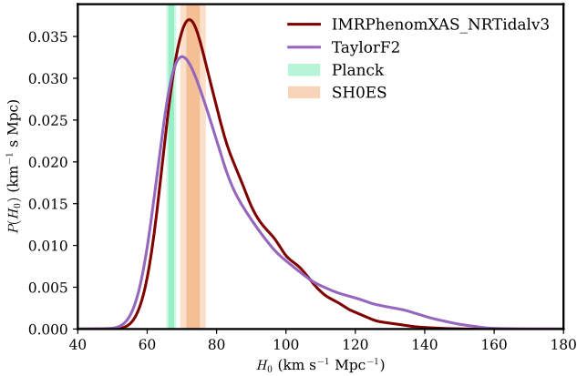
Figure 5. GW170817 H_0 posterior for IMRPhenomXAS_NRTidalv3 and TaylorF2 on the LVK-matched prior, shown as Silverman-bandwidth kernel-density estimates; the sample-derived 68 and 95 per cent HPDs (computed from the weighted samples, no KDE) are reported in Table 4. The Planck \Lambda CDM and SH0ES distance-ladder values are shown for context.
