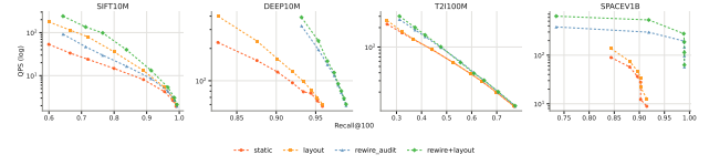
Figure 2: System ablation of static, layout-only, rewiring-only, and full PageWire variants.
