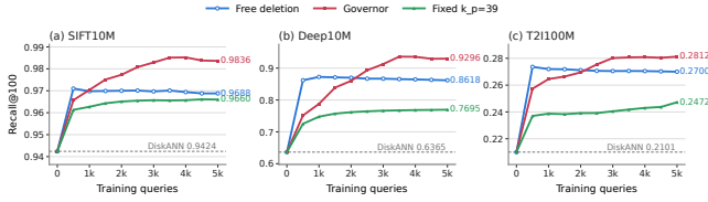
Figure 3: Recall during rewiring with free deletion and governed edge protection.
