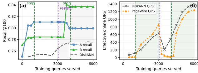
Figure 6: QPS and Recall comparison of Pagewire against DiskANN.
