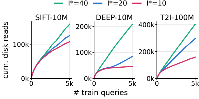
Figure 5: Effect of the target mean serving I/O I^* on cumulative traversal-sector reads during adaptation.
