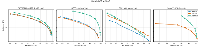
Figure 1: QPS-Recall comparison of PageWire, Starling and Margo.
