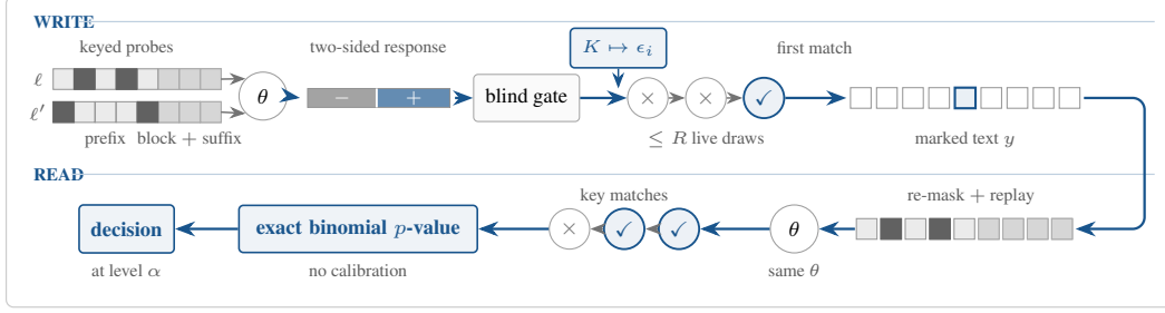
Figure 2: How Shibboleth writes a mark and reads it back. Keyed probes expose a two-sided response. The gate selects a carrier before the key reveals the accepted sign, then generation commits the first match. Verification re-masks the text, replays \theta , and returns an exact binomial p -value.
