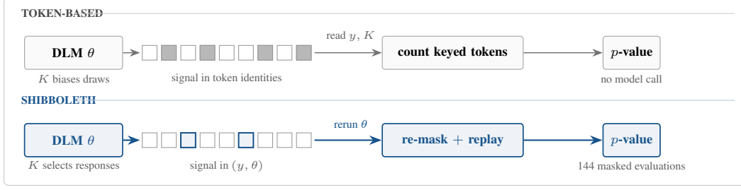
Figure 1: Two places to keep a watermark. Token-based methods store evidence in token identities and verify from y, K alone. Shibboleth stores evidence in the response of \theta to keyed context probes, so verification reruns the same checkpoint.
