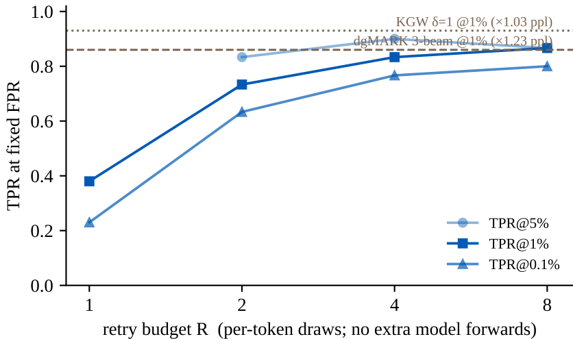
Detection vs retry budget (held-out, n=30, 512 tokens)
