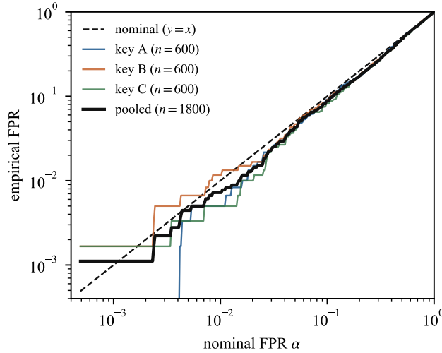
Figure 5: Empirical against nominal false-positive rate on human-written text. 600 C4 documents per key under three keys (pooled n = 1800 ), scored by the deployed verifier; the dashed line is exact calibration. Empirical rates track the nominal level across three orders of magnitude and sit at 0.043/0.0072/0.0011 at the 0.05/0.01/0.001 operating points.
