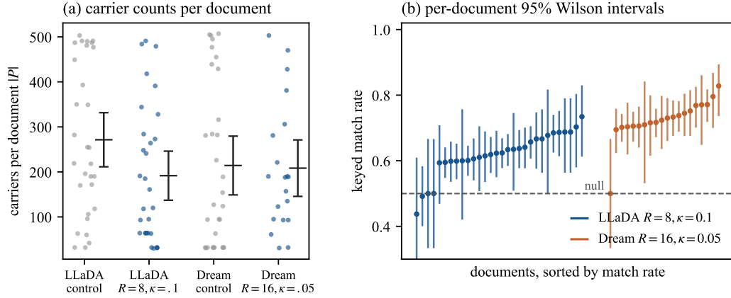
Figure 6: Per-document carrier counts and detection intervals. (a) Carrier pool size |P| per document for the control and watermarked arms of both models (dot = document; whisker = mean \pm 95\% CI). Counts range from about 30 to 500: short, EOS-padded documents admit few carriers. (b) Per-document 95% Wilson intervals on the keyed match rate for the watermarked arms, sorted; documents whose interval clears the 0.5 null carry individually decisive evidence, and the weakest documents overlap it.
