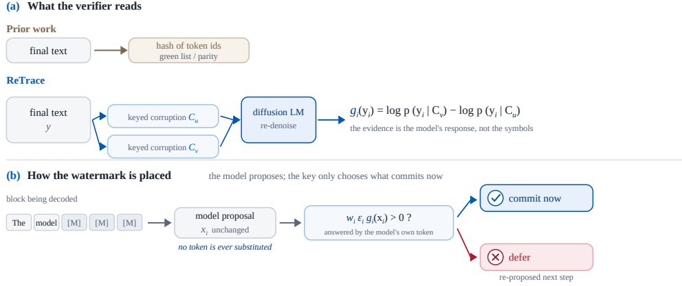
Figure 1: ReTrace embeds through the denoising trajectory but verifies through the model’s response to a keyed reconstruction. (a) Prior watermarks hand the verifier a function of the token identities — a green-list membership, a parity, a hash. ReTrace hands it the model: the finished text is corrupted twice under the key and re-denoised, and the contrast between the two reconstructions of the observed token is the evidence. The signal is therefore a property of the text’s relationship to the model rather than of its symbols, and it is recoverable from the text, the model and the key alone, with no access to the generation trajectory. (b) Placing it costs almost nothing because nothing is overridden. Decoding follows the reference block schedule and the model proposes what it would have proposed; the key decides only whether a proposal is committed now or deferred to a later step, when more of the block has resolved.
