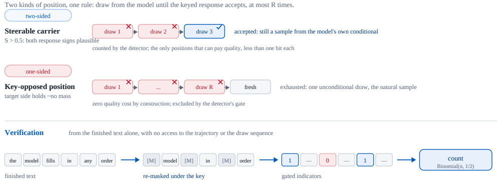
Figure 2: One rule, two regimes, and why the watermark is quality-free. At a steerable carrier both response signs are plausible, so a handful of redraws finds an accepting token that is still a sample from the model’s own conditional — these are the only positions that can pay quality, and each pays less than one bit by construction. At a key-opposed position every guided draw is rejected and the single unconditional fallback emits the natural sample: zero cost, and the detector’s gate excludes it. The verifier needs neither the trajectory nor the draw sequence: it re-masks the finished text under the key, reads one gated indicator per carrier, and counts against an exact Binomial( n, \frac{1}{2} ) null.
