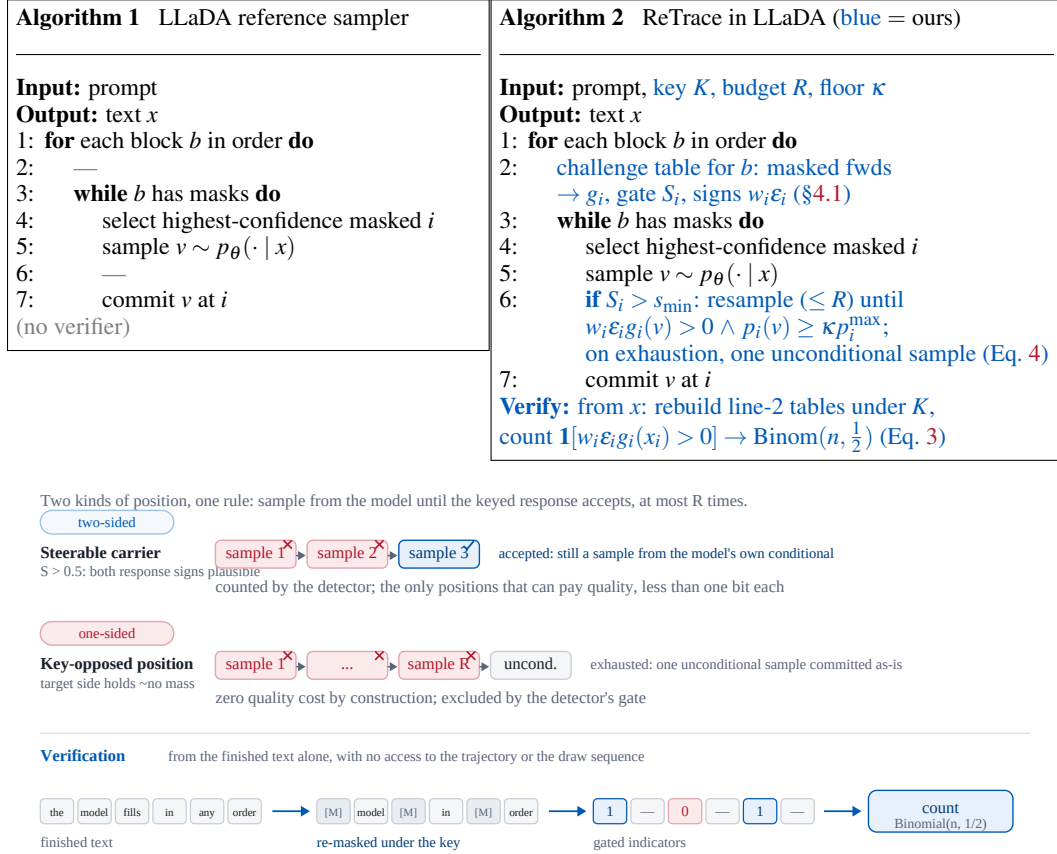
Figure 2: One rule, two regimes. A two-sided carrier accepts within a few resamples — still a sample from the model’s conditional, and the only kind of position that pays quality. A key-opposed position rejects every proposal and commits the natural sample at zero cost; the gate excludes it. The verifier re-masks under the key and counts gated indicators against an exact binomial null, with no access to the trajectory.
