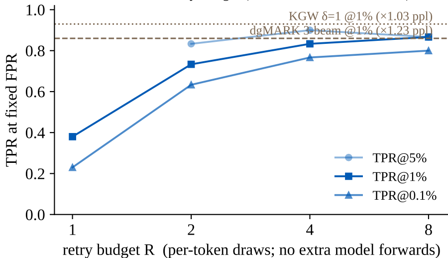
Detection vs retry budget (held-out, n=30, 512 tokens)
